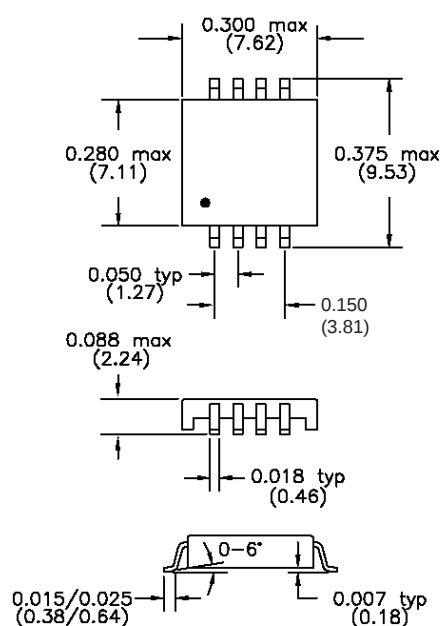
P3 Package
