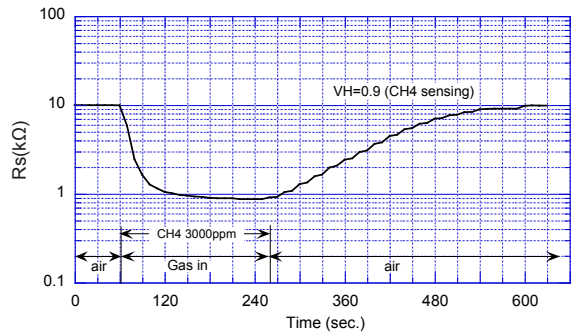
Figure 8a - Gas response speed - methane
