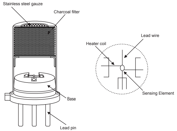
Figure 1 - Sensor structure
