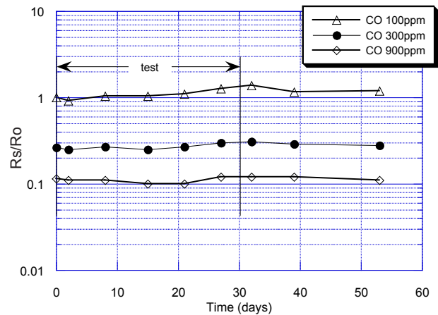
Figure 11b - Effects of exposure to 30ppm CO for 30 days (Ro= Rs in 100ppm CO prior to CO exposure, VH =0.2)
