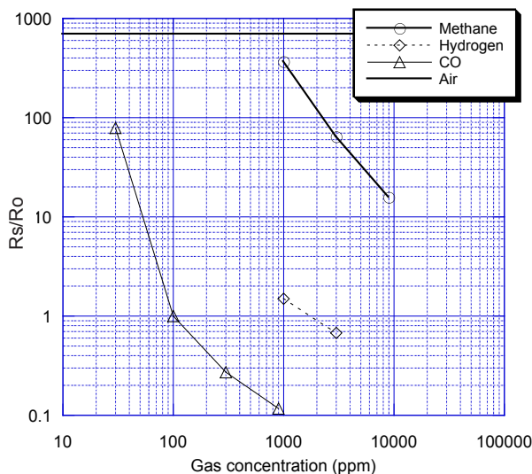
Figure 5b - Sensitivity to various gases for CO sensing (Ro = Rs in 100ppm of CO, VH =0.2)
