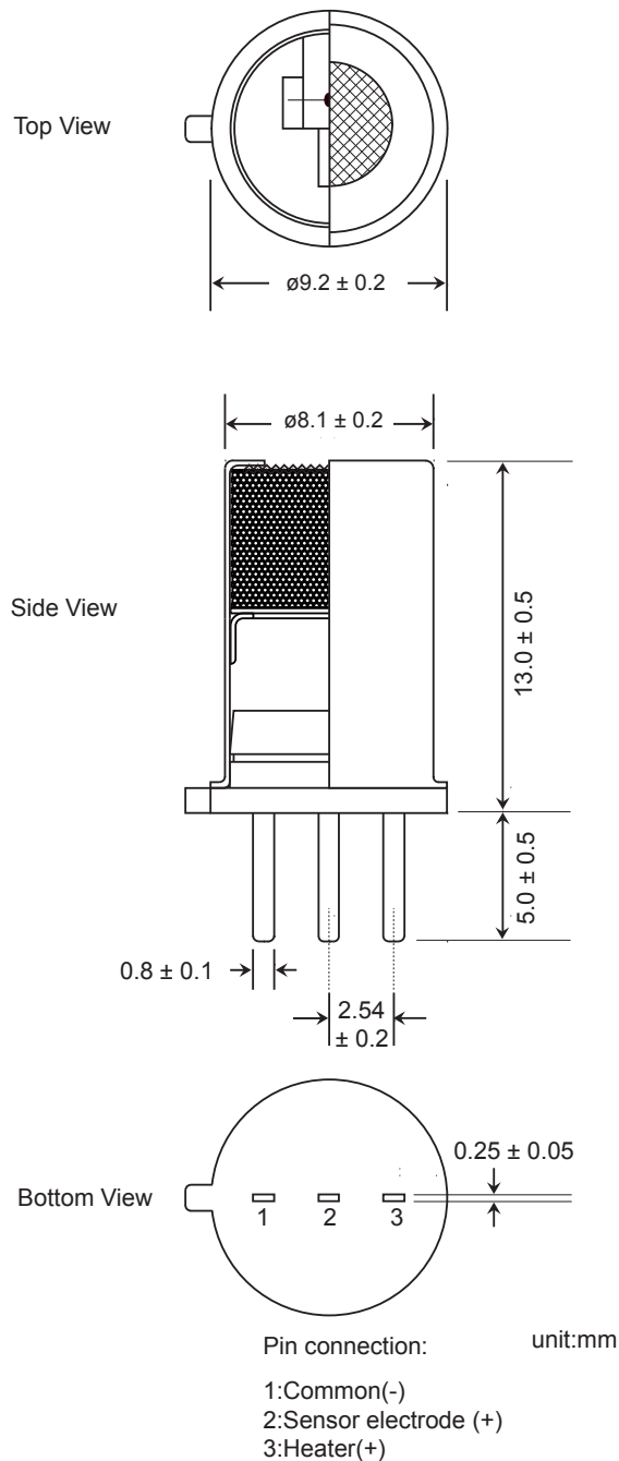
Figure 3 - Dimensions
