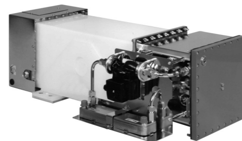
solid-state magnetron modulator
