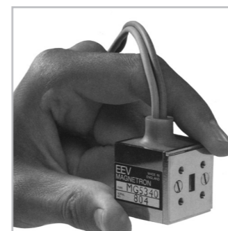
Miniature KA(Q)-Band pulse magnetron
