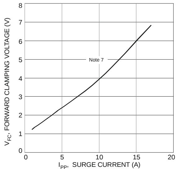
Fig. 4 Typical Forward Clamping Characteristics
