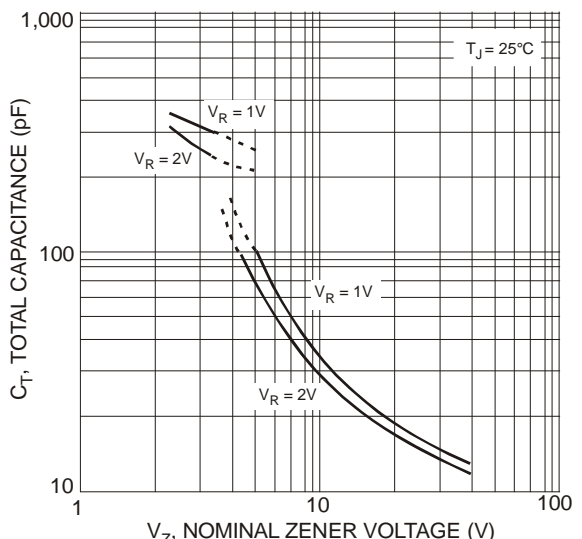
Fig. 5 Typical Total Capacitance vs. Nominal Zener Voltage
