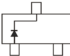
BAT54W Marking: KL5
