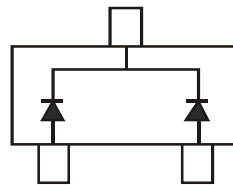
BAT54CW Marking: KL7
