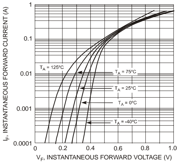
Fig. 1 Forward Characteristics
