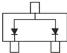
BAT54AW Marking: KL6
