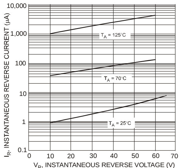
Fig. 4 Typical Reverse Characteristics, B350B thru B360B
