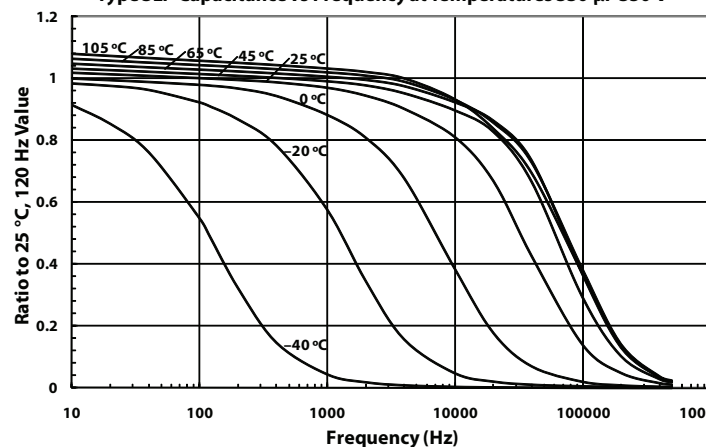
Type SLP Capacitance vs Frequency at Temperatures 330 \mu F 350 V
