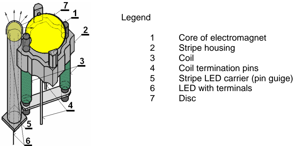
Pict.1. Use DOT-LED principle cell
