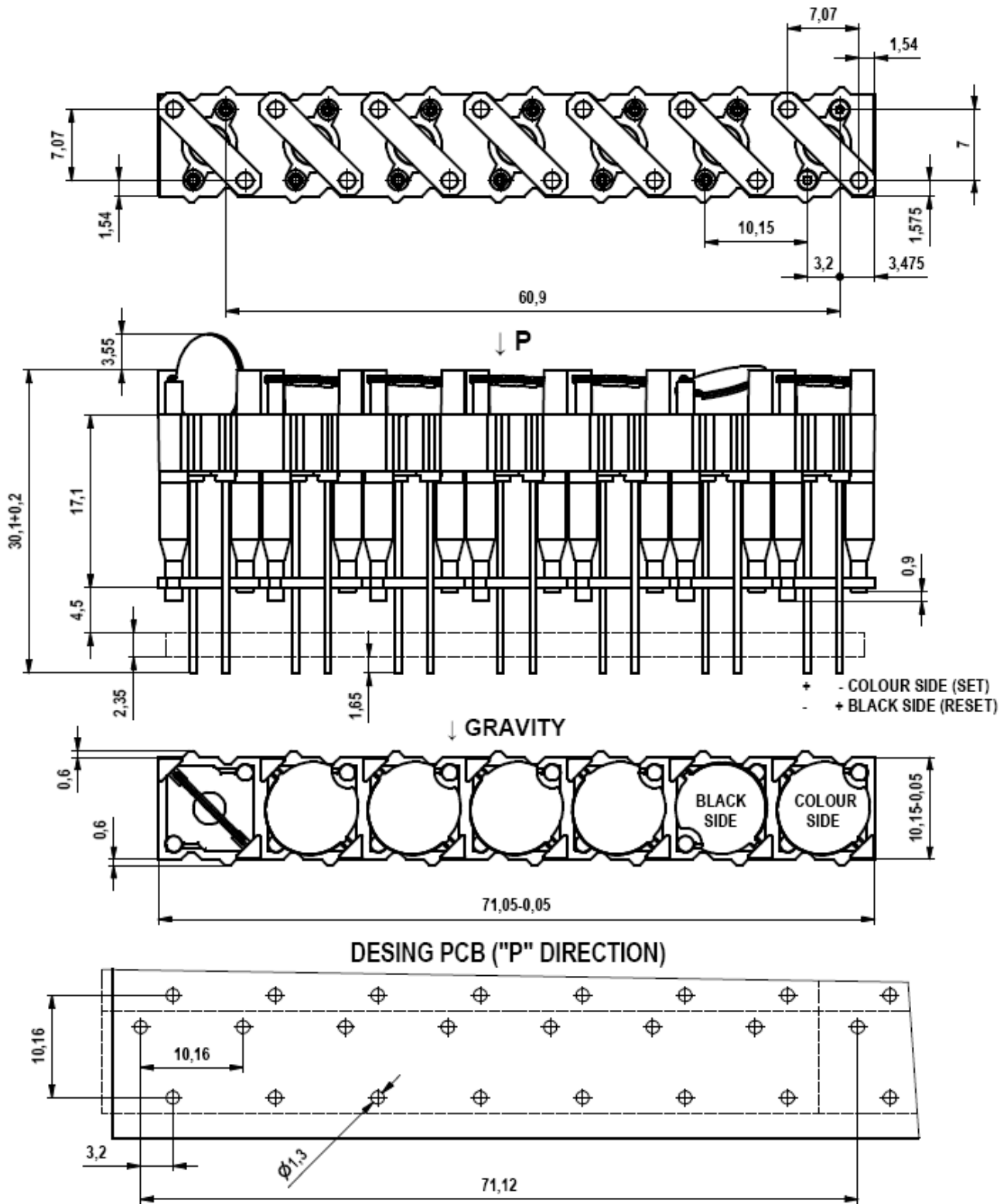
Pict.4. Layout and basic dimensions of BS 1005
