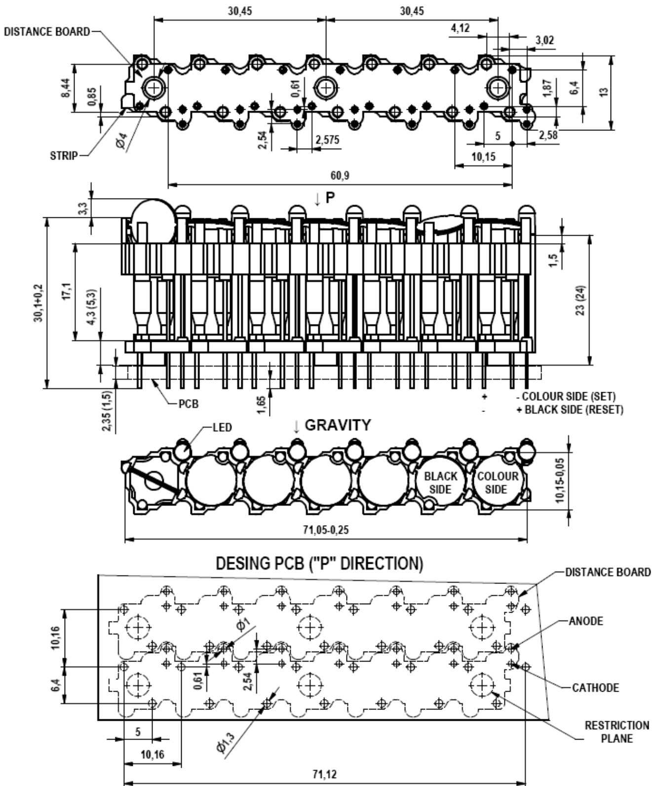
Pict.3. Layout and basic dimensions of BS 1004
