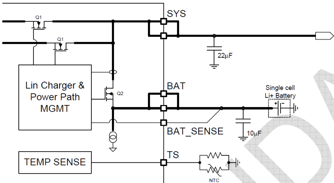
Figure 27. Battery Circuitry
