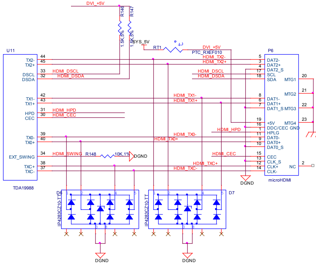
Figure 44. Connector Interface Circuitry
