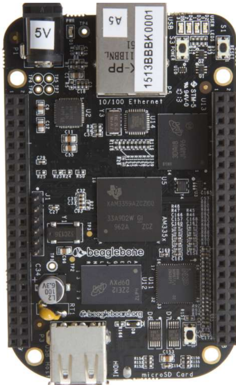
Figure 69. Top Side
