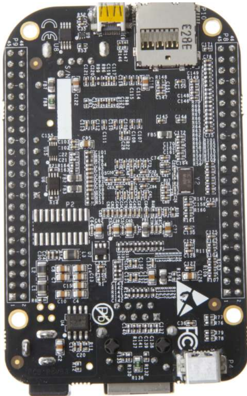
Figure 70. Bottom Side
