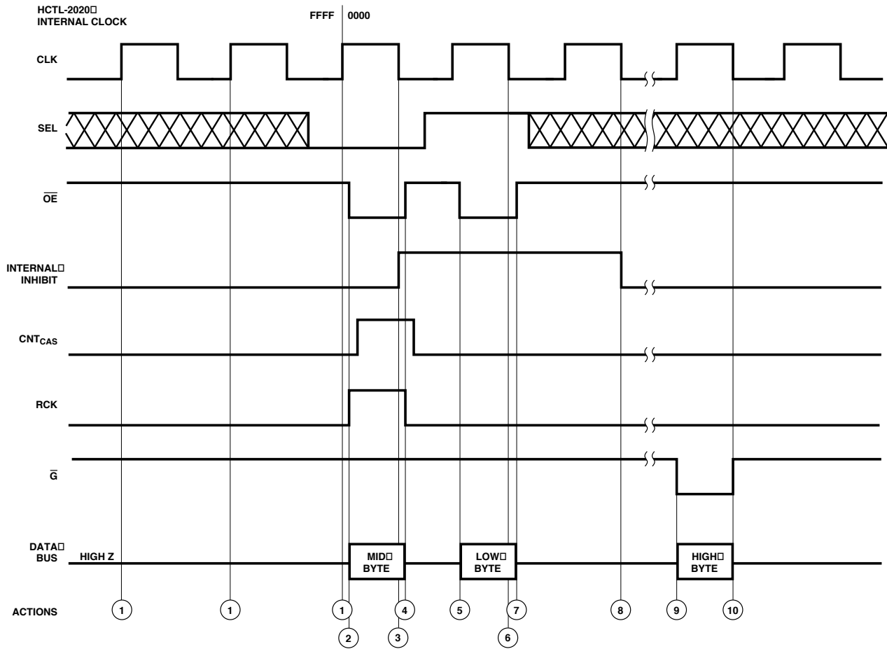
Figure 16. Interface Timing for the 6802/8.
