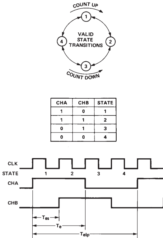
Figure 9. 4x Quadrature Decoding.
