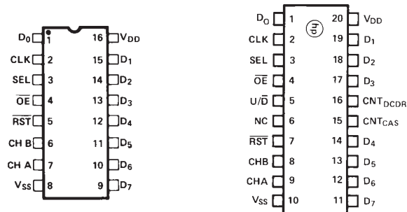
PINOUT A
