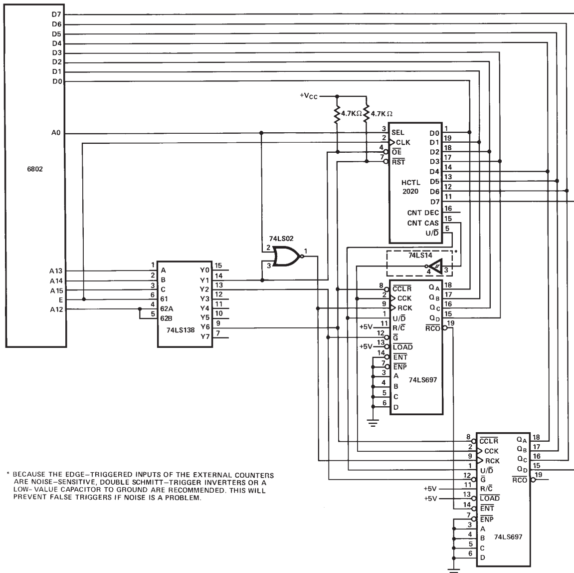
Figure 14. A Circuit to Interface to the 6802/8.
