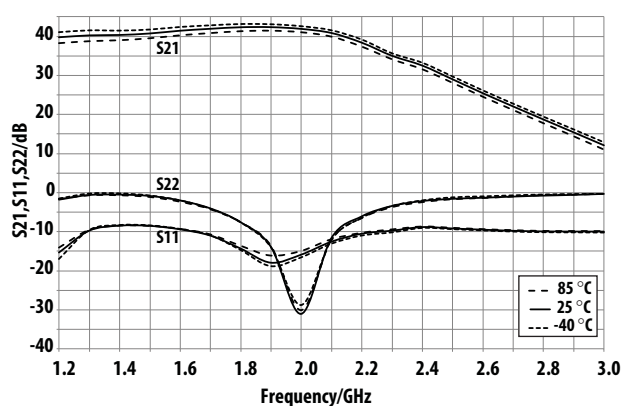
Figure 6. Small-signal performance Over-temperature V_{dd}=V_{ddBias}=5.5V operating voltage
