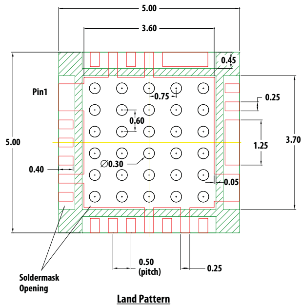
Land Pattern
