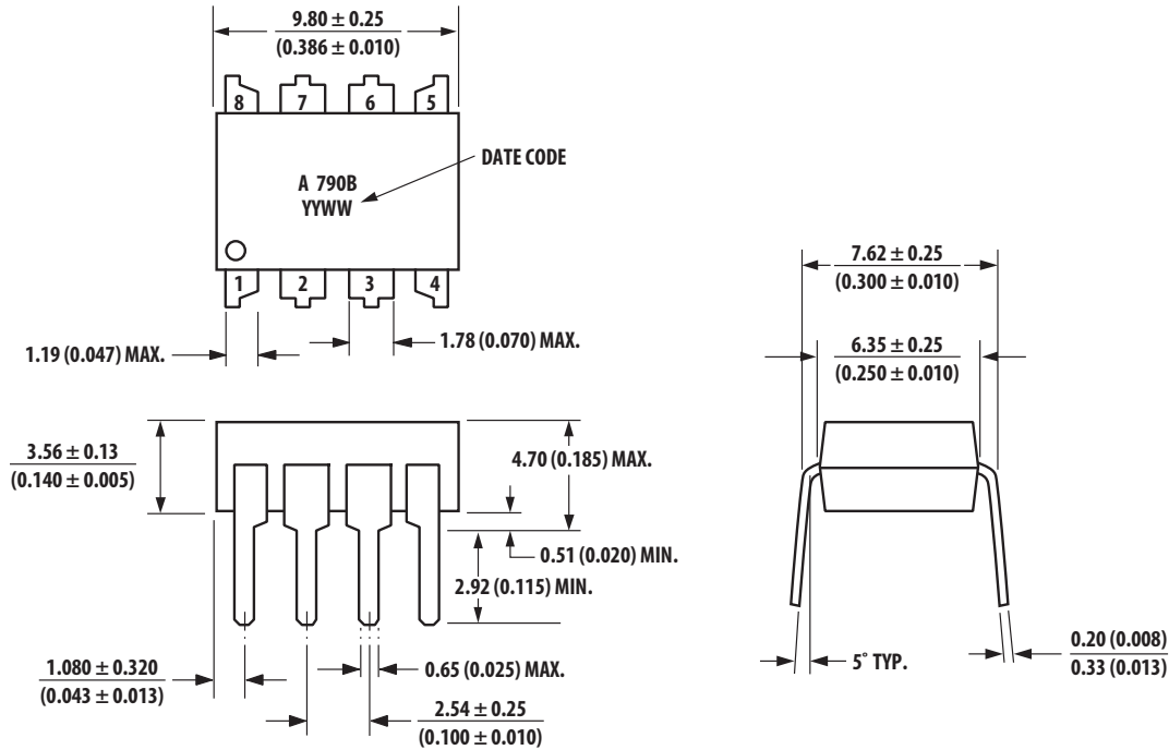
Figure 1. Standard DIP Package
