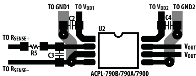
Figure 22. Example printed circuit board layout.
