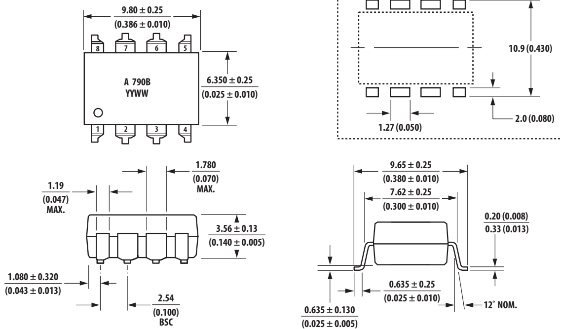
Figure 2. Gull Wing Surface Mount Option 300
