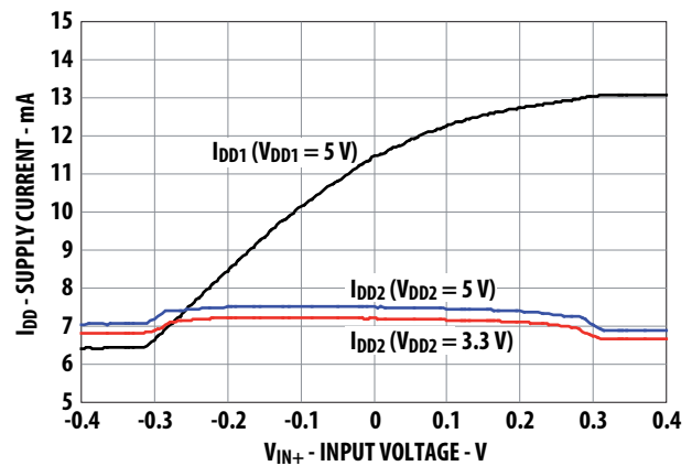
Figure 20. Supply current vs. input voltage.
