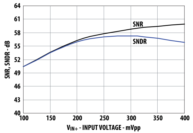
Figure 16. SNR, SNDR vs. input voltage.
