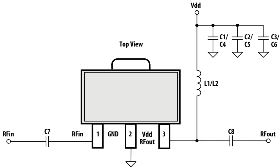
Figure 30. Application Schematic
