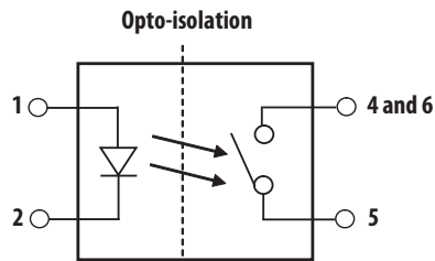
Equivalent Relay Diagram
