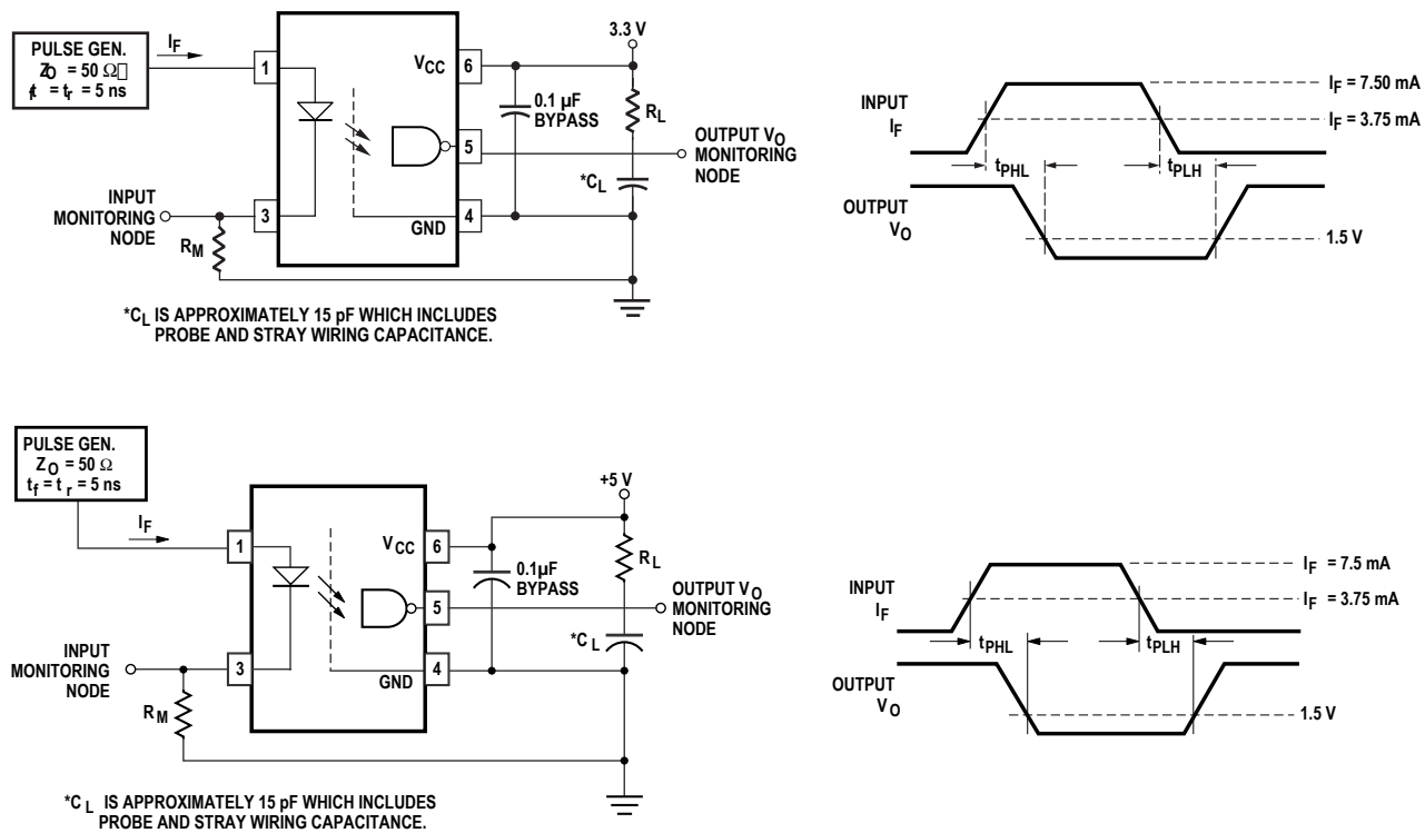
Figure 6. Test circuit for t_{PHL} and t_{PLH} .
