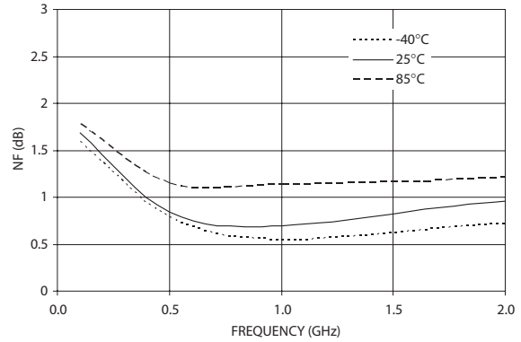
Figure 26. NF vs. Frequency (5V 10mA)
