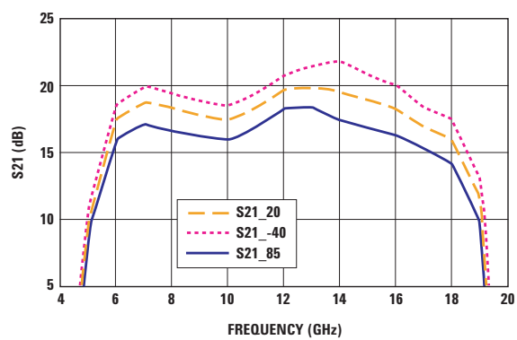
Figure 14. Typical gain over temperature
