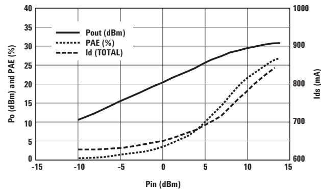
Figure 5. Typical output power, PAE, and total drain current versus input power at 8 GHz
