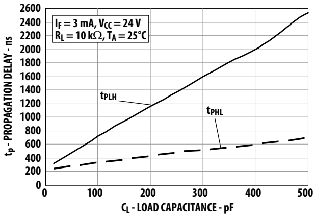
Figure 11. Typical Propagation delay vs. Load Capacitance
