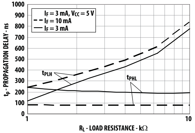
Figure 10. Typical Propagation Delay vs. Load Resistance
