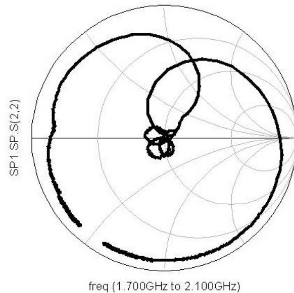
Figure 6. S(2,2)
