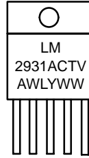
TO-220 T SUFFIX CASE 314D
