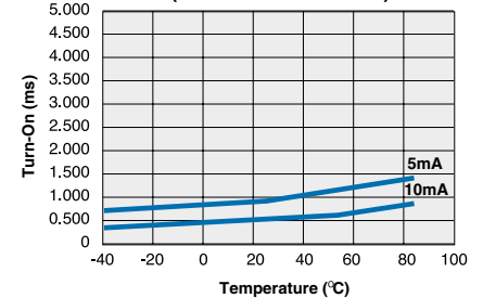
CPC1135N Typical Turn-On vs. Temperature (Load Current = 50mA)
