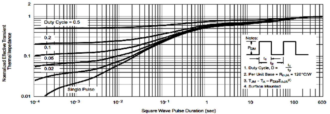
Fig 12: Normalized Thermal Transient Impedance, Junction-to-Ambient
