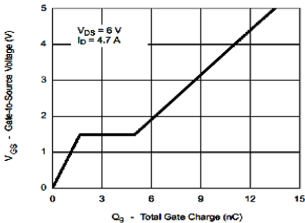
Fig 3: Gate Charge
