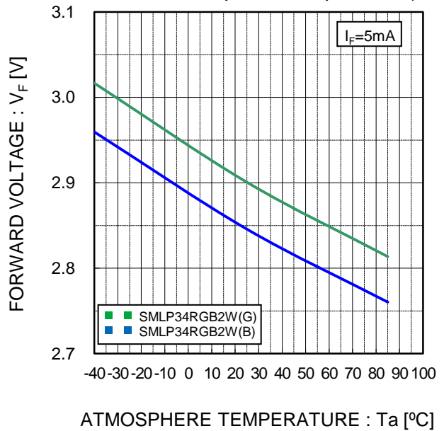
Fig.2-2 Forward Voltages - Atmosphere Temperature (G, B)
