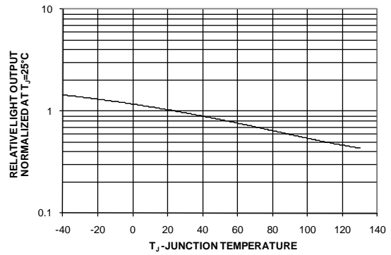
Figure 6: Relative Light Output vs Junction Temperature
