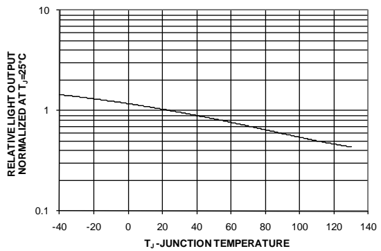
Figure 6: Relative Light Output vs Junction Temperature
