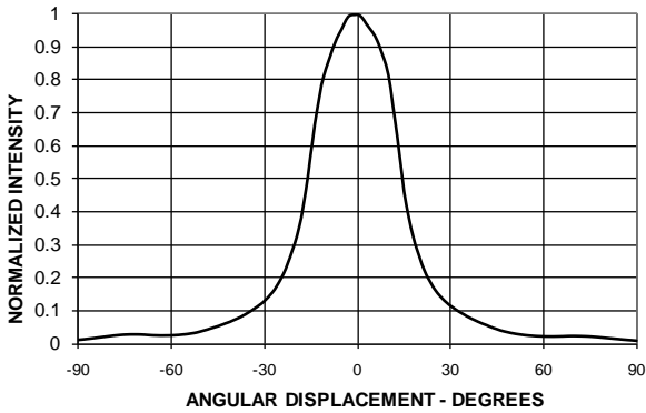
Figure 5: Representative Radiation pattern for 30° Viewing Angle Lamp
