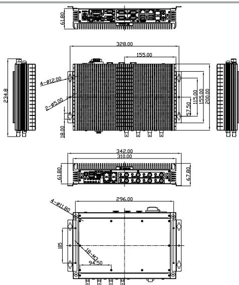
TANK-700-QM67
