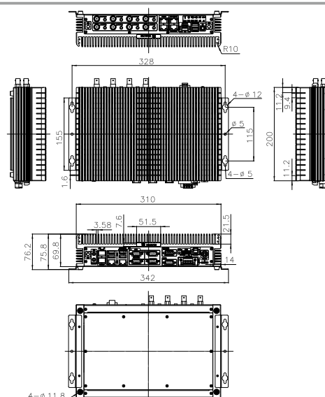
TANK-720-Q67
