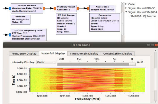
The GNU Radio application running the BB60C analyzer as a flowgraph block.
