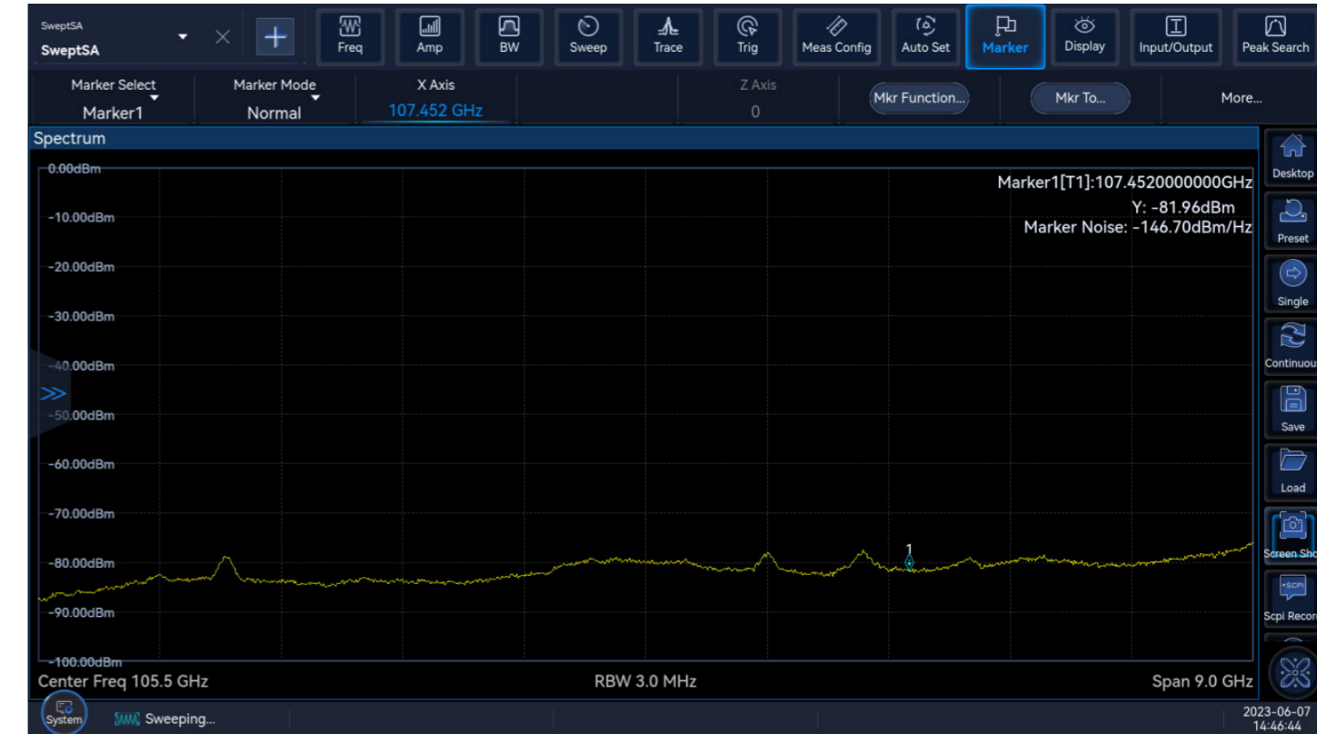
101GHz to 110GHz frequency band DANL specification
